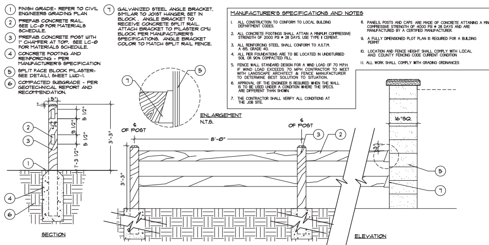
Fig. 3-33A 3'-3" Concrete Split Rail Fence (Phase 1A only)
