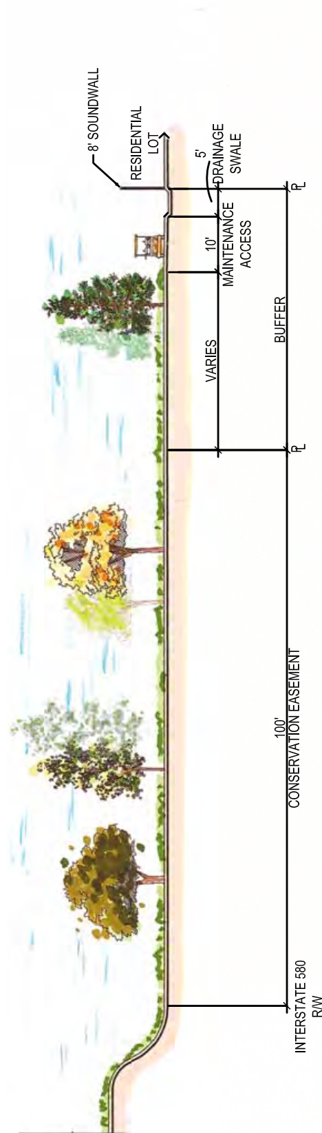
Figure 3-15 SECTION B
