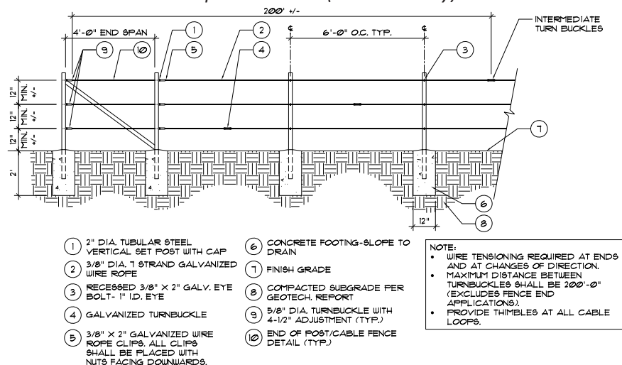
Fig. 3-33B 3'-3" Post and Cable Fence
