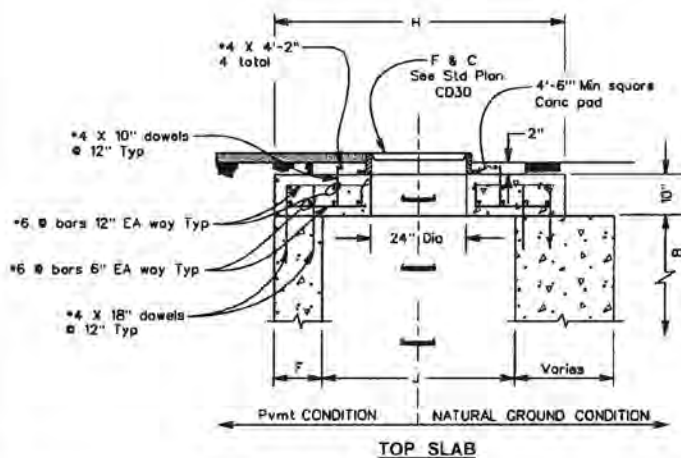
TOP SLAB
