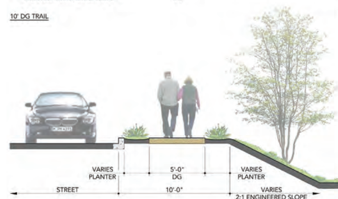
DG TRAIL ALONG I-580
