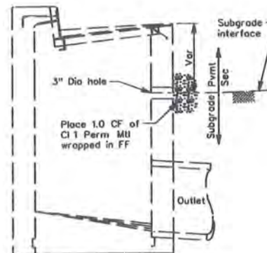
STANDARD FRONTSIDE WEEPHOLE DETAIL See Note 3
