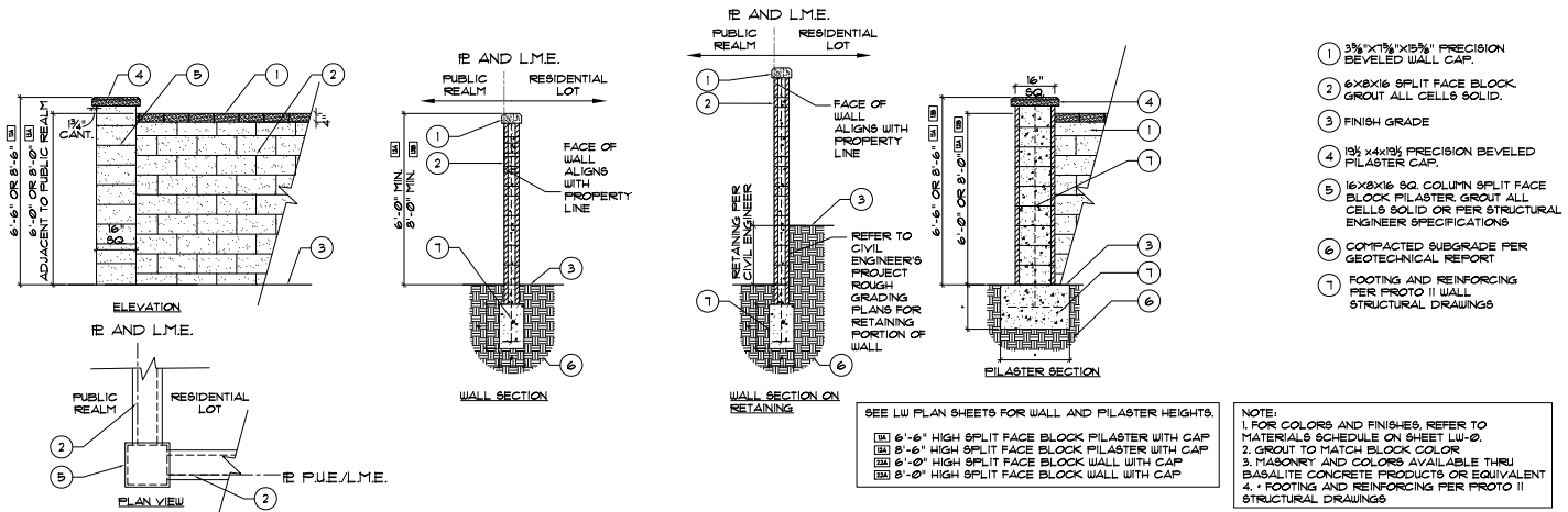
Fig. 3-32 8'-0" Split Face Block Wall with Cap Color: Eco Brown or equal
