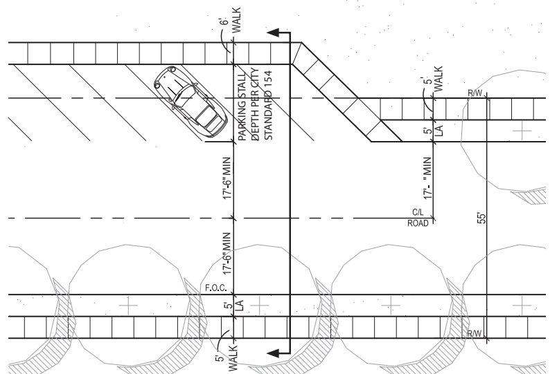
Figure 3-26 Public Park Angled Parking Street Section and Plan View
