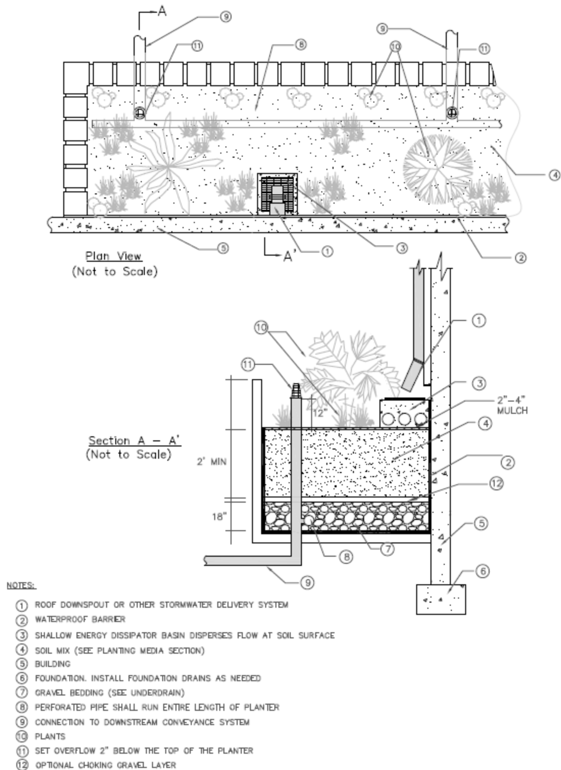
Figure F-4. Example Stormwater Planter Schematic
