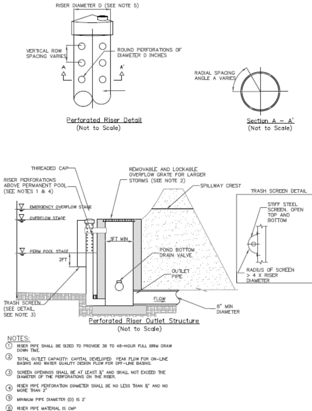
Figure F-13. Riser Outlet Schematic
