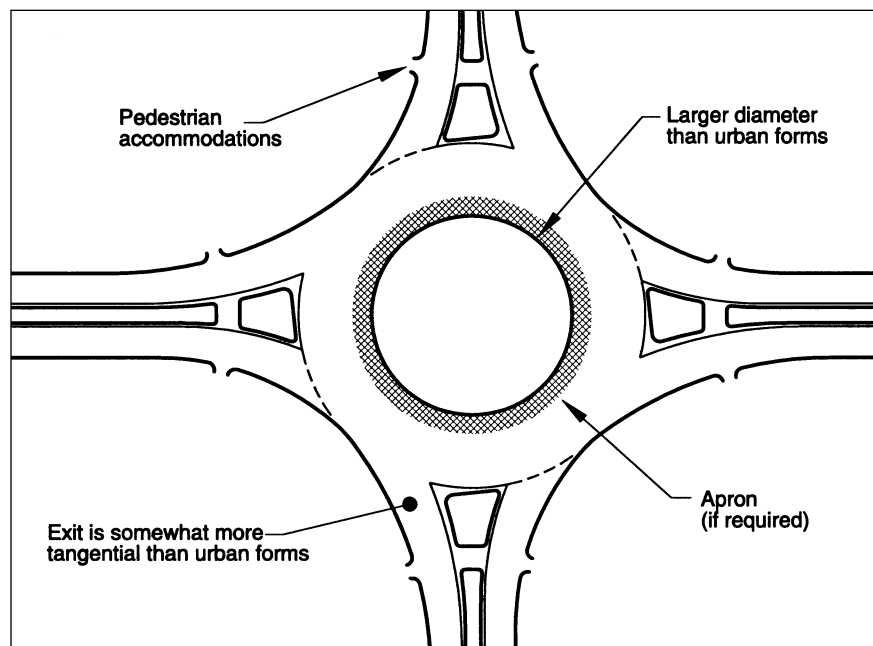
Exhibit 1-12. Typical rural single-lane roundabout.
