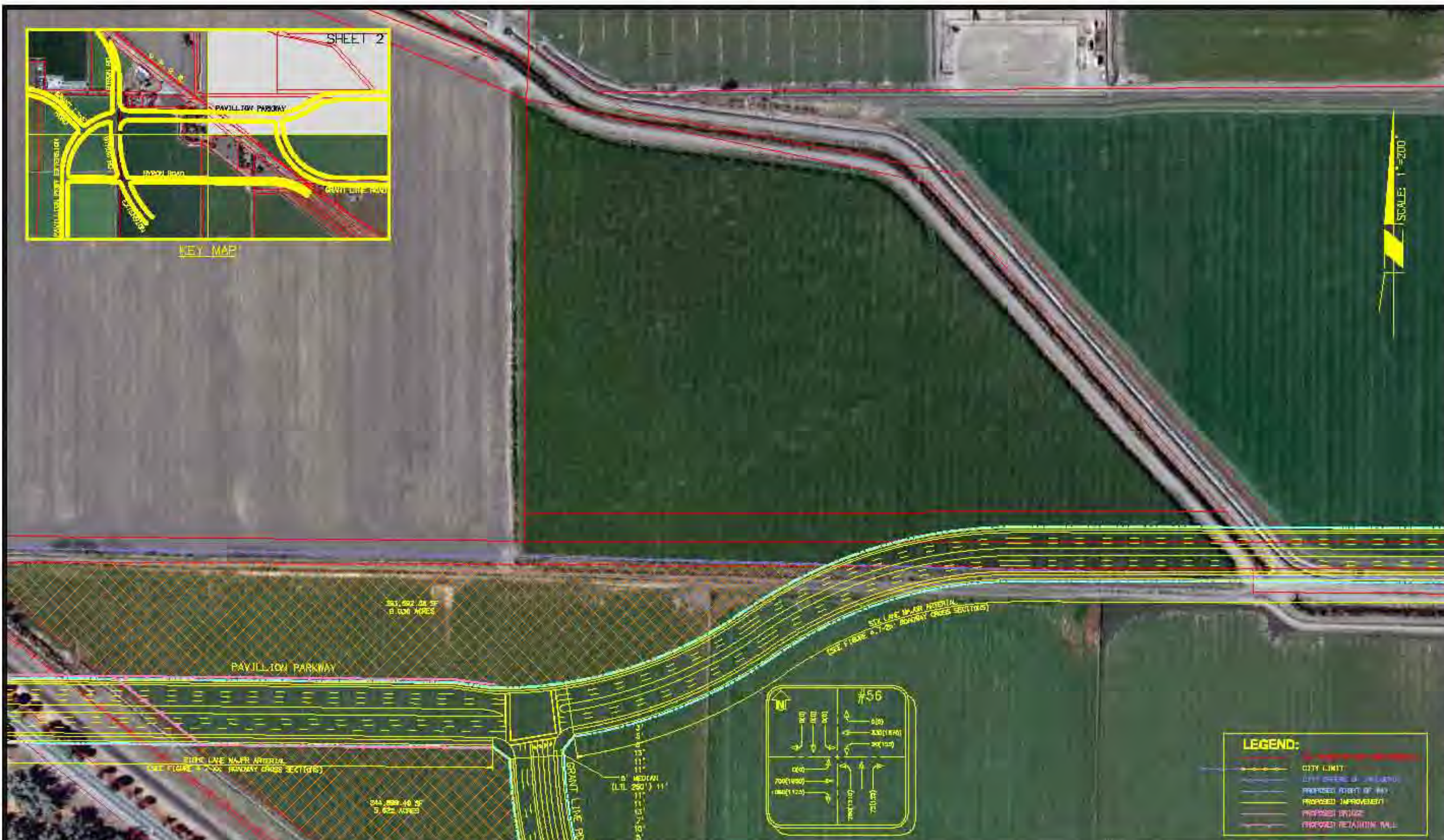
CONCEPT PLANS FOR INTERSECTION #56 PAVILLION PARKWAY & GRANT LINE ROAD (SHT 2 OF 4) UPDATED 11-05-2010
