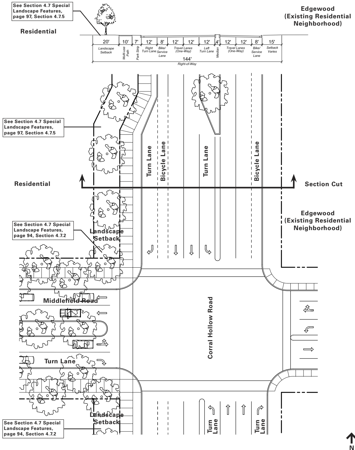
FIGURE 4.23 Build-out Section and Plan: Regional Arterial – Corral Hollow Road, Designation B (Final Build-out)
