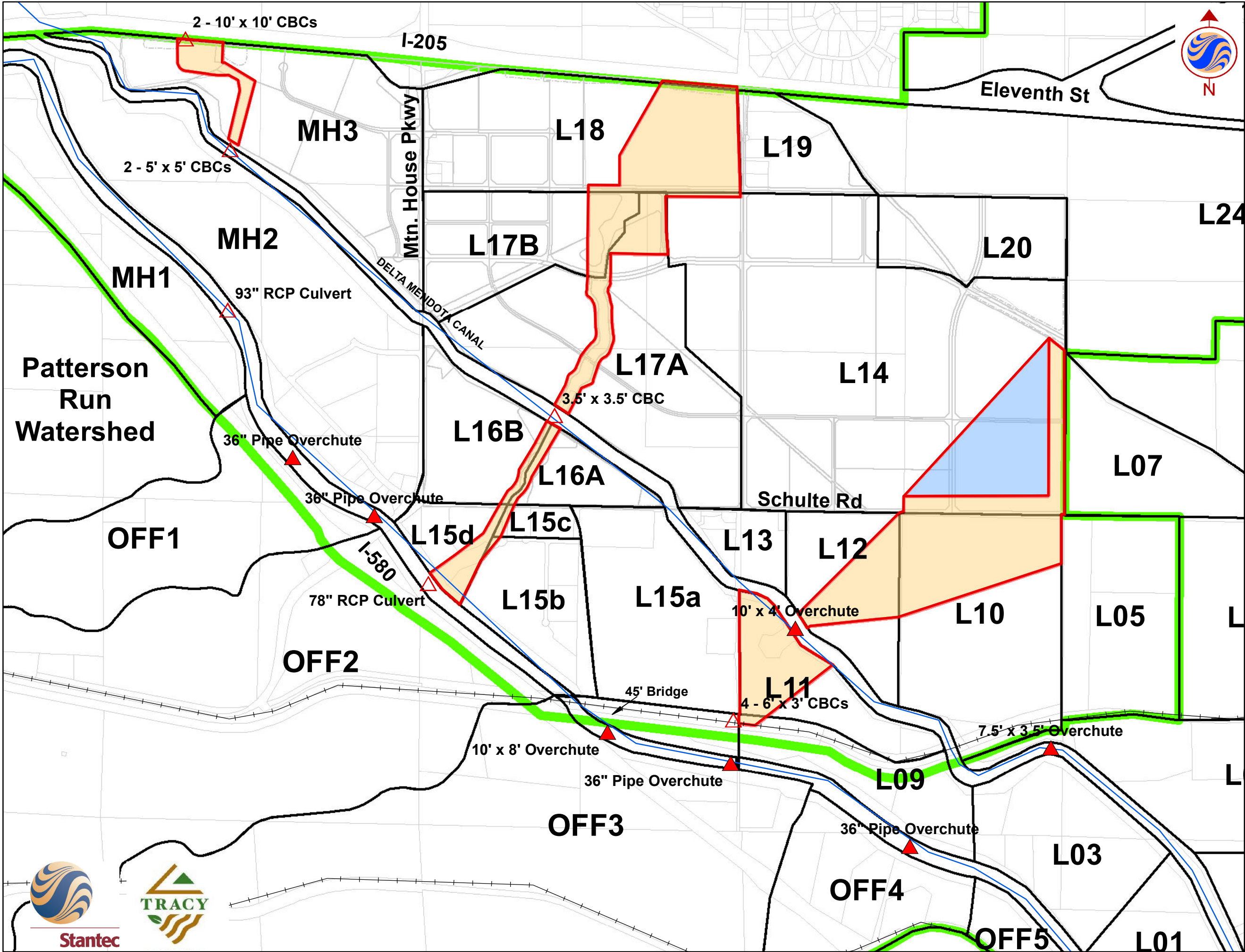
FIGURE 5-8 AREAS REQUIRING SPECIAL HYDROLOGIC & HYDRAULIC CONSIDERATION DUE TO INFLOWS FROM OFFSITE WATERSHEDS NOVEMBER 2012 184010207 SCALE 1" = 1500'
