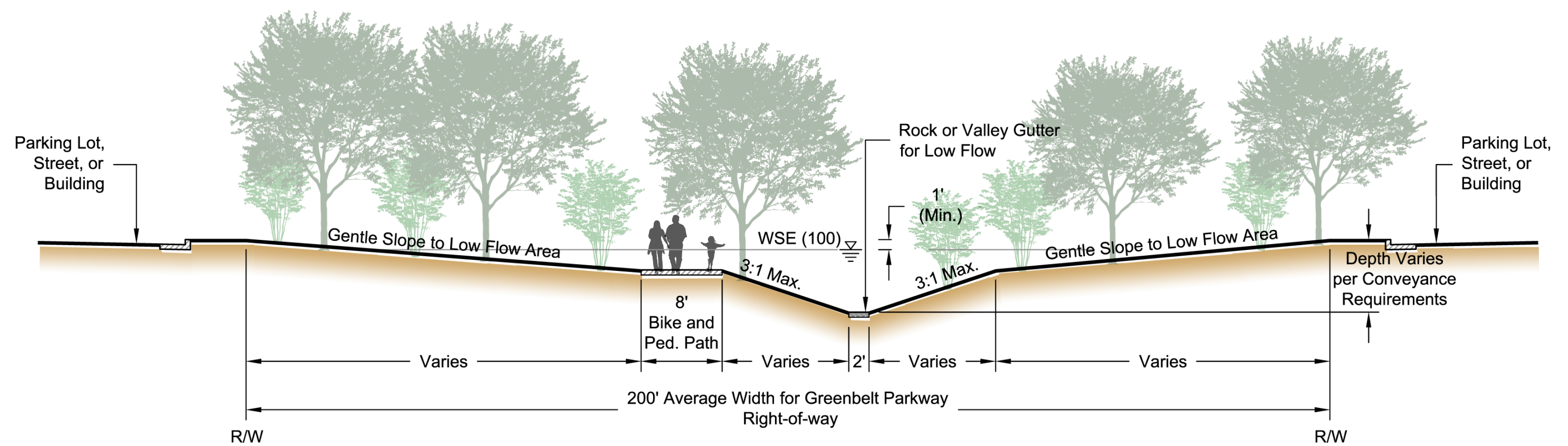
Greenbelt Parkway Typical Cross-Section
